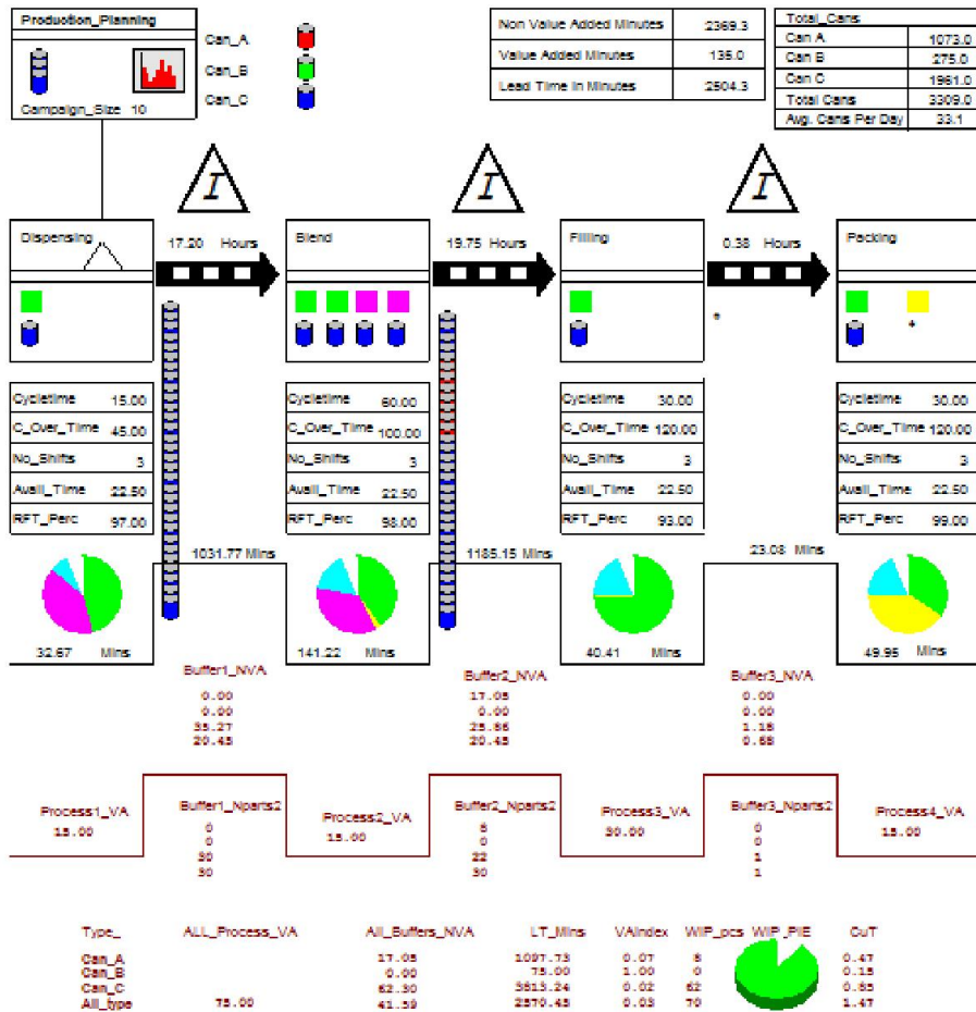
Fig. 4 Completed VSM model - WITNESS Power with Ease 2.0 VSM_Witness.mod
