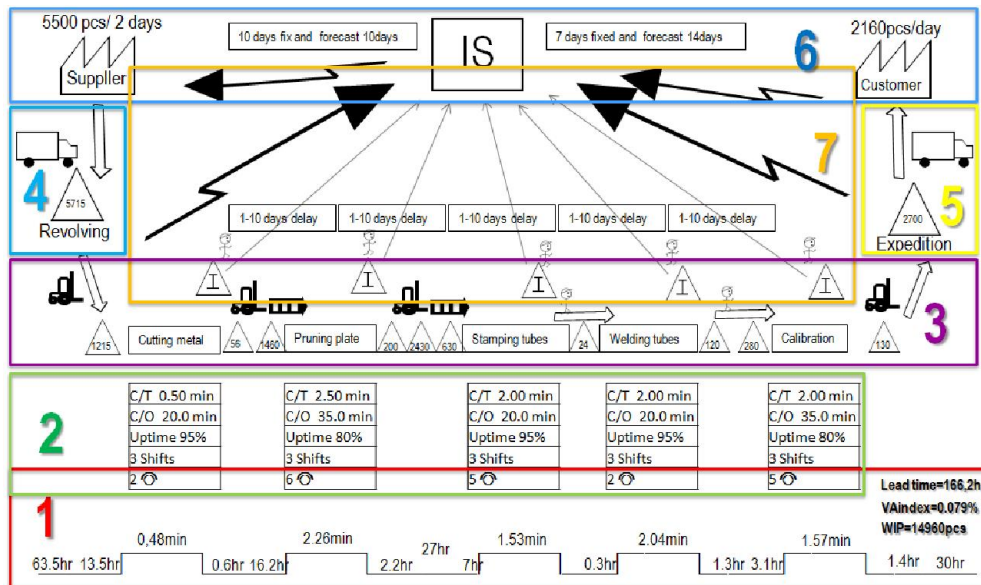
Fig. 1 VSM key stones – Value stream mapping
